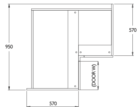
0666 L Shape Corner Base 0667 950W L Shape Corner Base with Carousel
