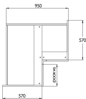
0666/0667 L Shape Highline Corner 3/4 Carousel 950W
