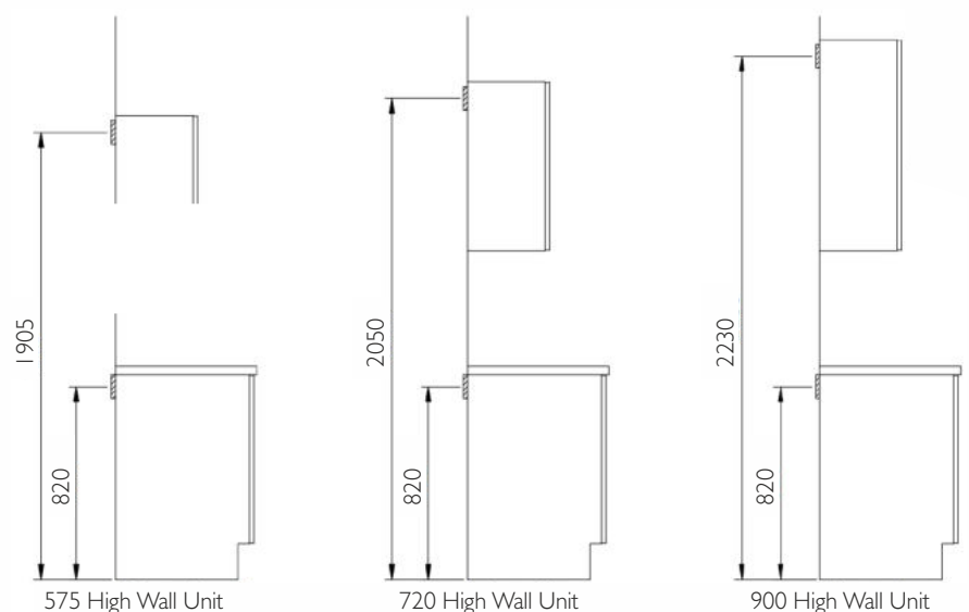
Pattress Position for Wall Fixings
