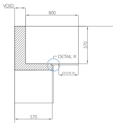
Corner Base Unit Planning 800W
