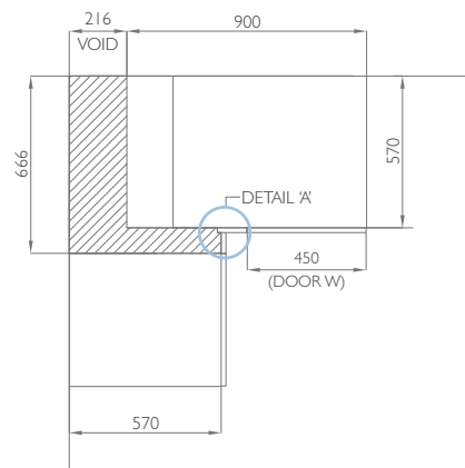
Corner Base Unit Planning 900W
