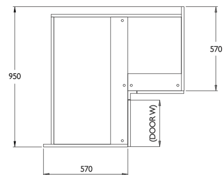
95HLLCB L Shape Corner Base 95HLLCBCA 950W L Shape Corner Base with Carousel
