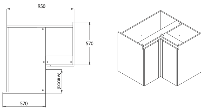
95HLLCB/95HLLCBCA L Shape Highline Corner 3/4 Carousel 950W
