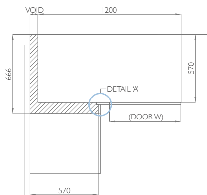
Corner Base Unit Planning 1200W
