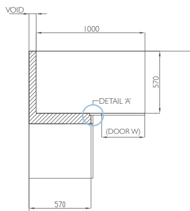
Corner Base Unit Planning 1000W
