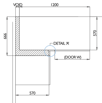
Highline Corner Units
